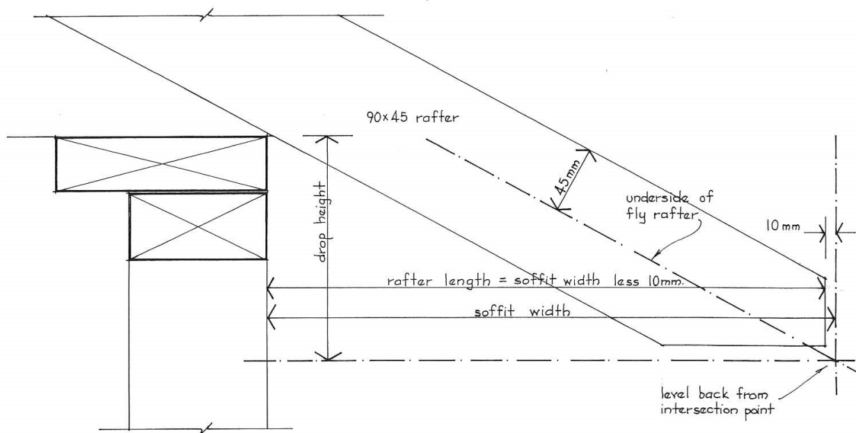
CONCRETE TILE ROOF - SET OUT
