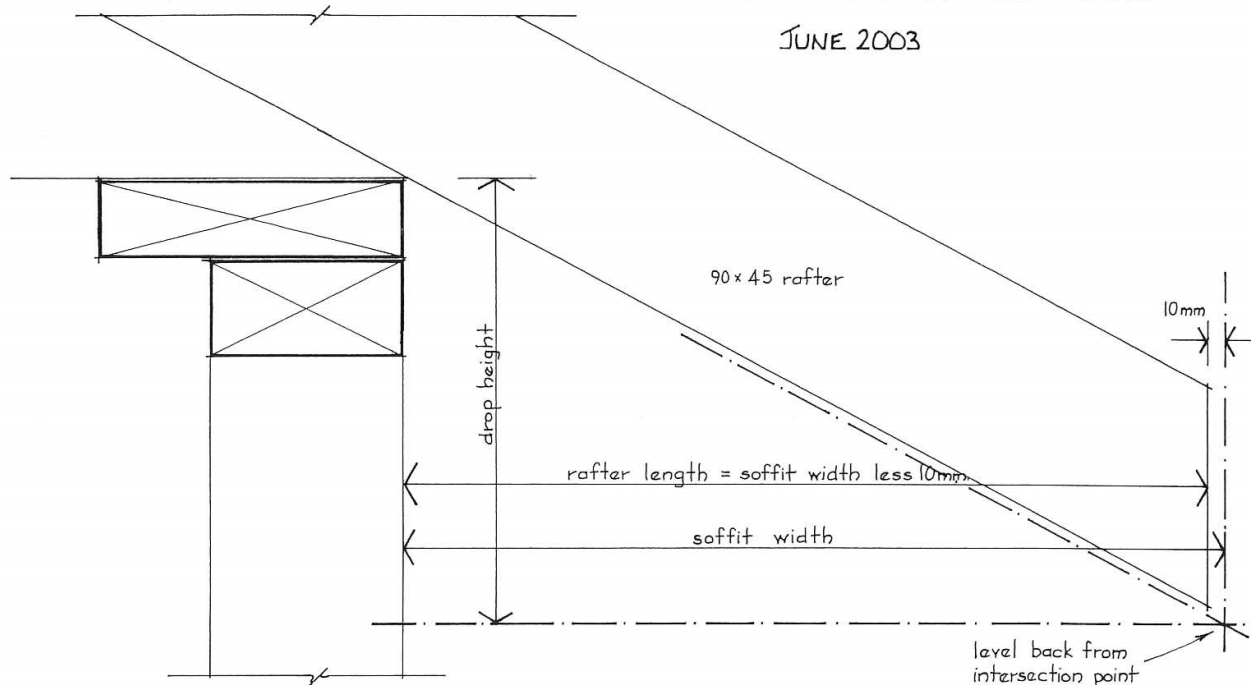
METAL ROOF - SET OUT
